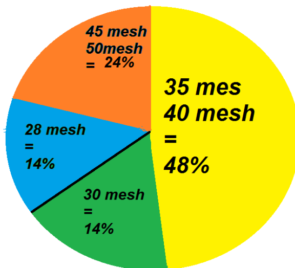
Percentage and level of dispersion of grading Edible salt
